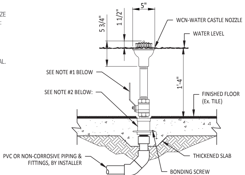
ELEVATION VIEW
